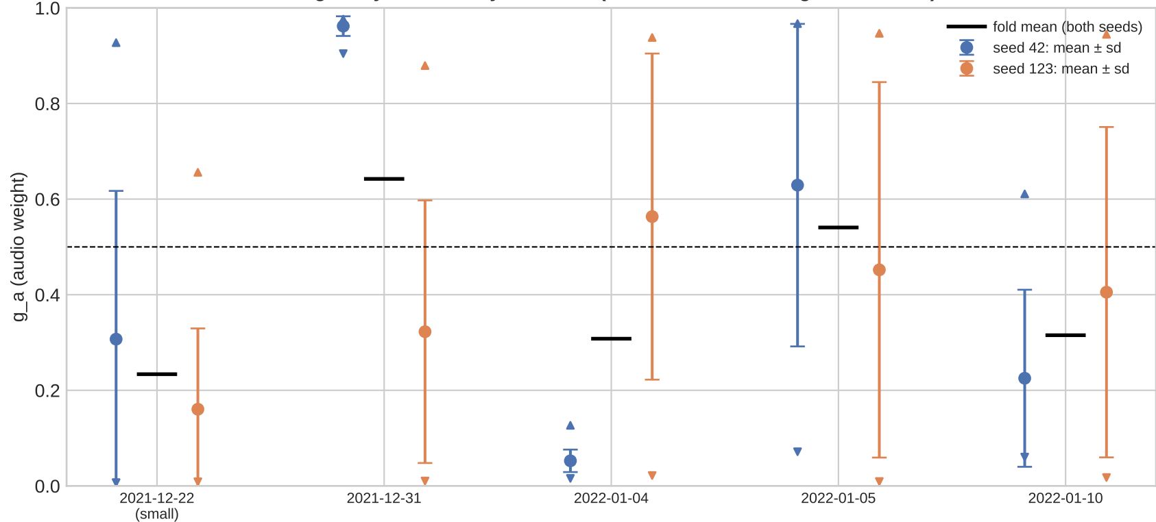
F1 gate by unseen day and seed (blue = seed 42, orange = seed 123)
